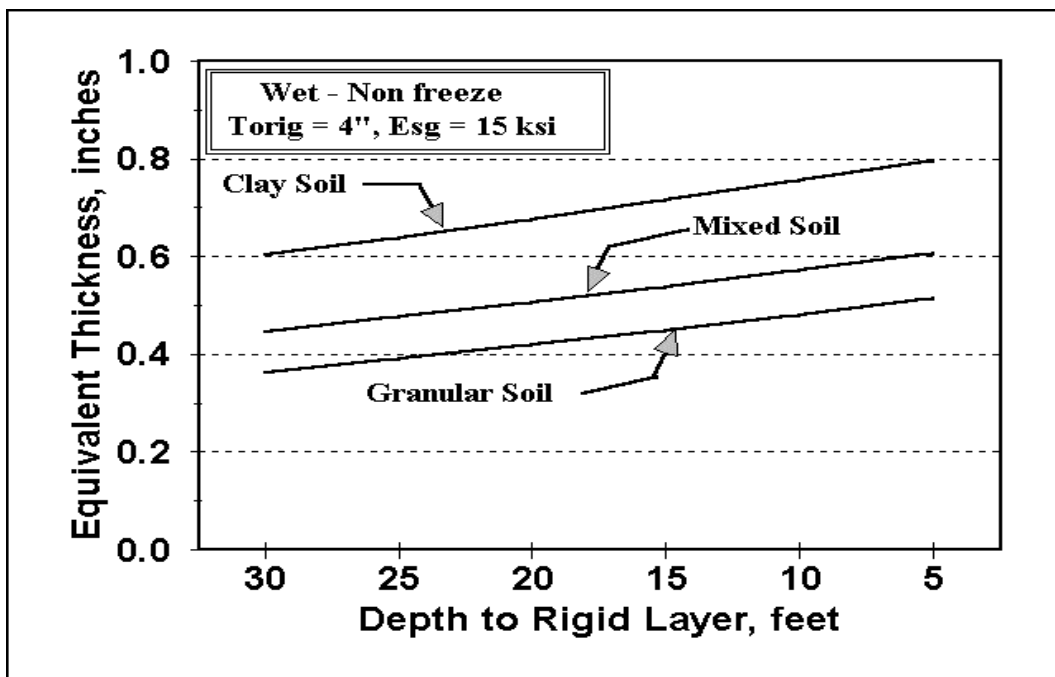
Figure 23. AC/Fabric Equivalent Thickness ( Amount of Reduction in AC Overlay Thickness) Nomograph for Wet-Non Freezing Zones
